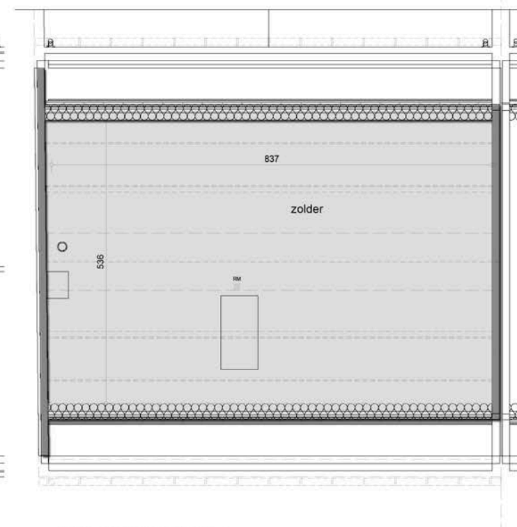
ZOLDERVERDIEPING
