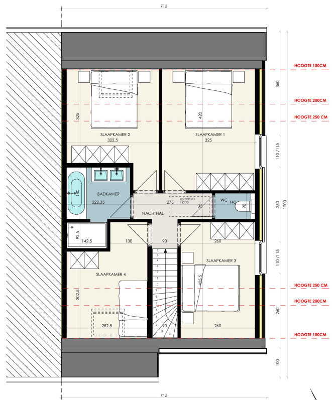
VERDIEPING LOT 3
